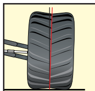
Positive Camber
